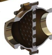
DN50 Bronze ConstaFlo Sectioned View
