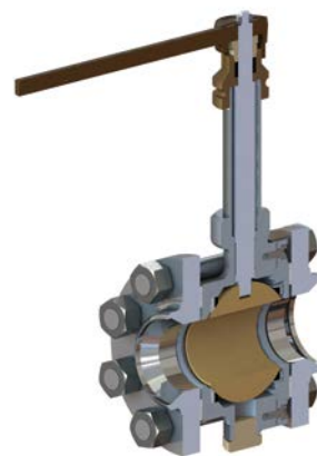
Sectioned View
